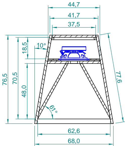
Section B-B
